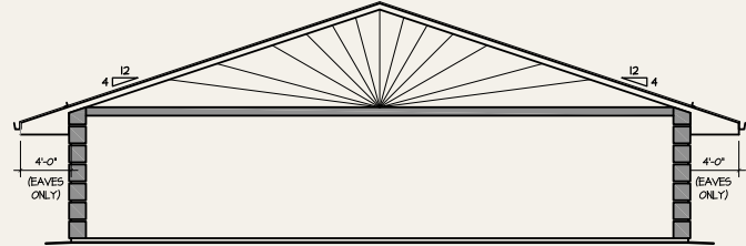
Building Elevation 1/8" = 1'-0"
