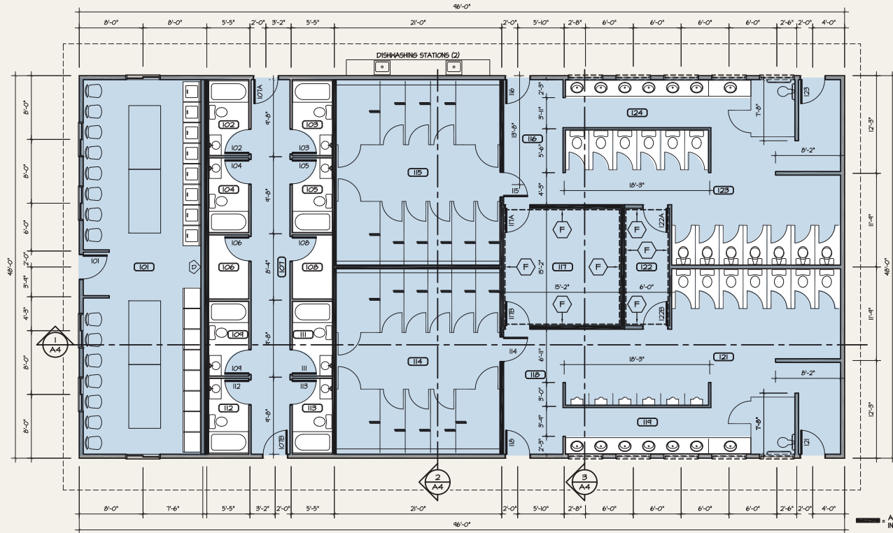
1 Floor Plan A2 1/8" = 1'-0" 4608 sq. ft. (428 m 2 )
